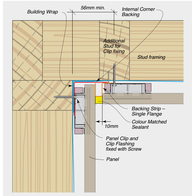
FIGURE 8.10 Internal Corner Detail – With Backing Strip and Colour Matched Sealant – Plan View
