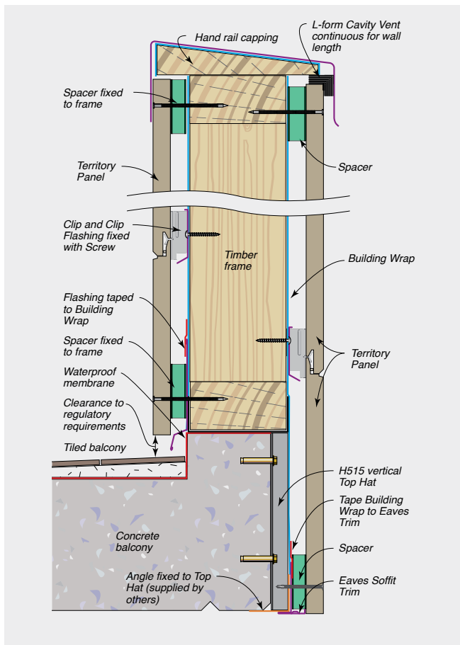
FIGURE 8.36 Typical Balcony Rail
