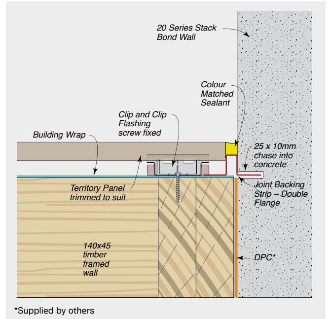
FIGURE 8.30 Internal Corner Junction Panel/Bond Wall
