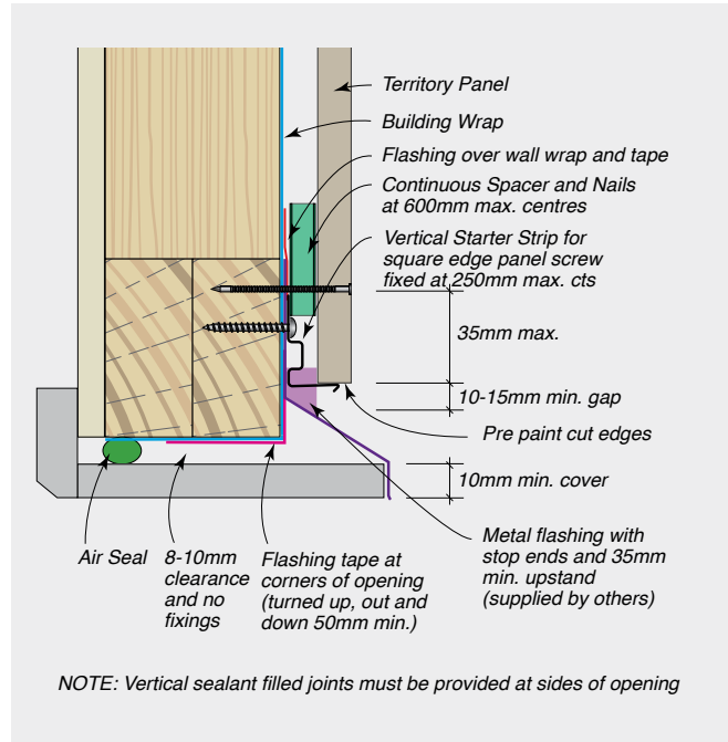
FIGURE 8.24 No Soffit wall detail
