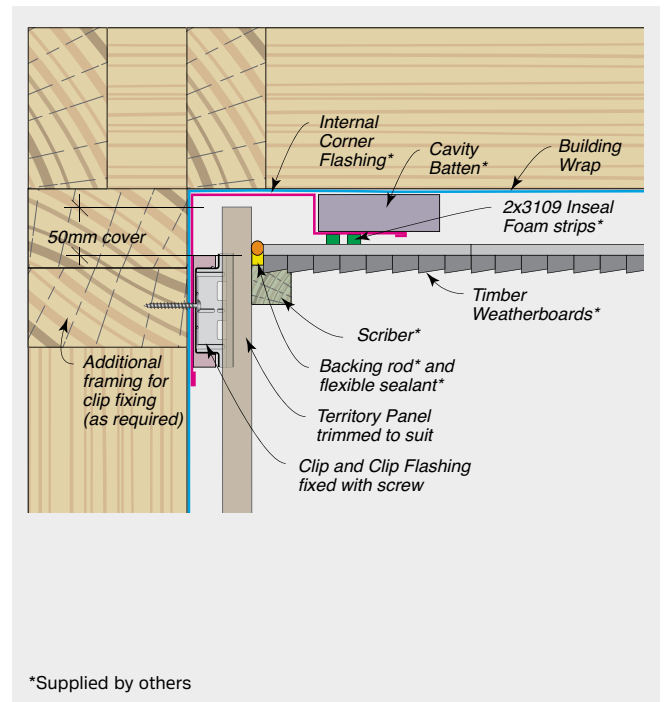
FIGURE 8.32 Internal Corner Junction Panel/Weatherboard
